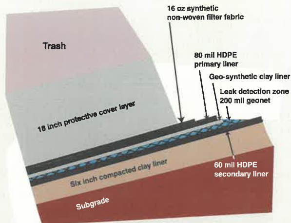
Pioneer Crossing Landfill Typical liner detail
