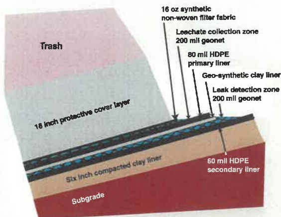
Pioneer Crossing Landfill Typical liner detail
