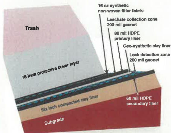
White Pines Landfill Typical liner detail
